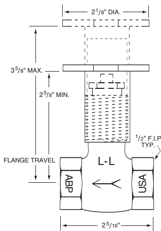
Straight Valve Diagram
