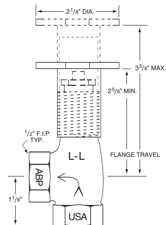
Angle Valve Diagram
